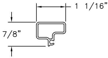
MEETING RAIL REINFORCEMENT (11585) ALUMINUM 6063-T5
